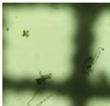
Gambar 4. Oscillatoria sp.
