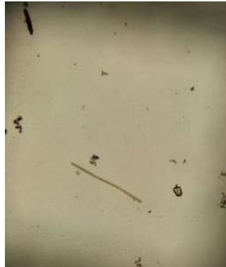
Gambar 5. Trichodesmium sp.
