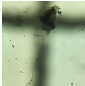
Gambar 8. Hapalosiphon sp.
